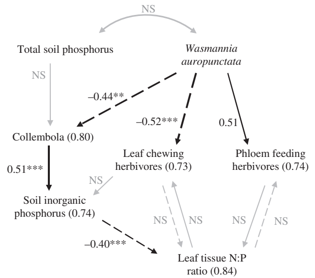
Figure 4 Results of a path analysis evaluating the effects of Wasmannia auropunctata invasion on soil inorganic phosphorus and leaf nutrients. Arrows represent direction of interaction. Dashed lines indicate negative effects and solid lines indicate positive effects. The numbers by the arrows represent interaction strengths (path coefficients) and numbers in parentheses represent the proportion of variance not explained by the model (error variance). Grey lines represent non-significant (NS) interactions, which were not included in the final model. * P < 0.05 , ** P < 0.01 , *** P < 0.005 .
